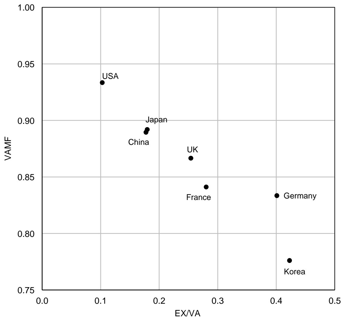
Figure 15. Relationship between VAMF and the share of total exports in GDP
