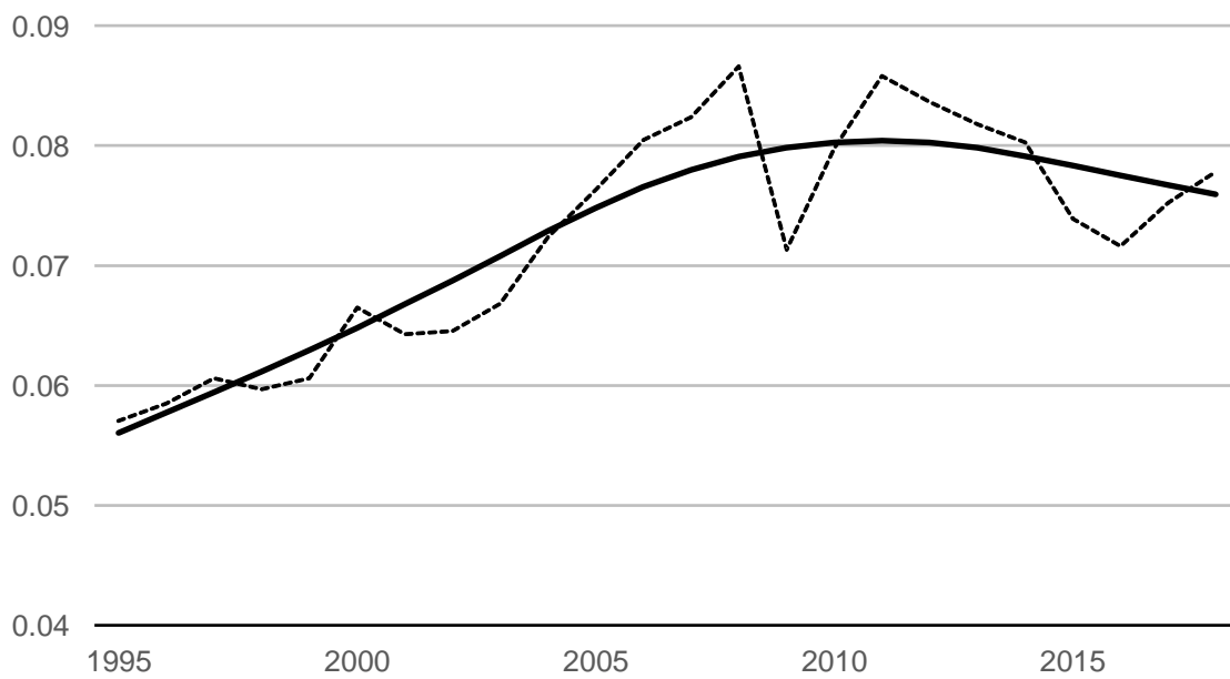
Figure 18. Share of Imported intermediate Input out of Total Cost ( a^m )
